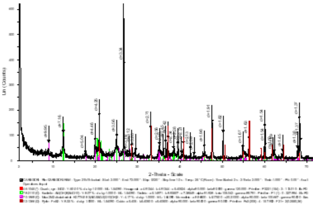
Figure 2 X-ray diffraction of Coal Mining Reject.
