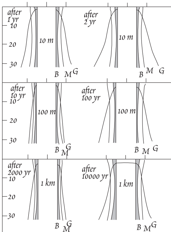
Figure 12.19. Temperatures as a function of time and distance surrounding basaltic dikes of various thickness. Lines B, M, and G are the temperatures of biotite breakdown, muscovite breakdown and granite minimum melting respectively. Gray area is region of partial melting. From Patchett (1980).
