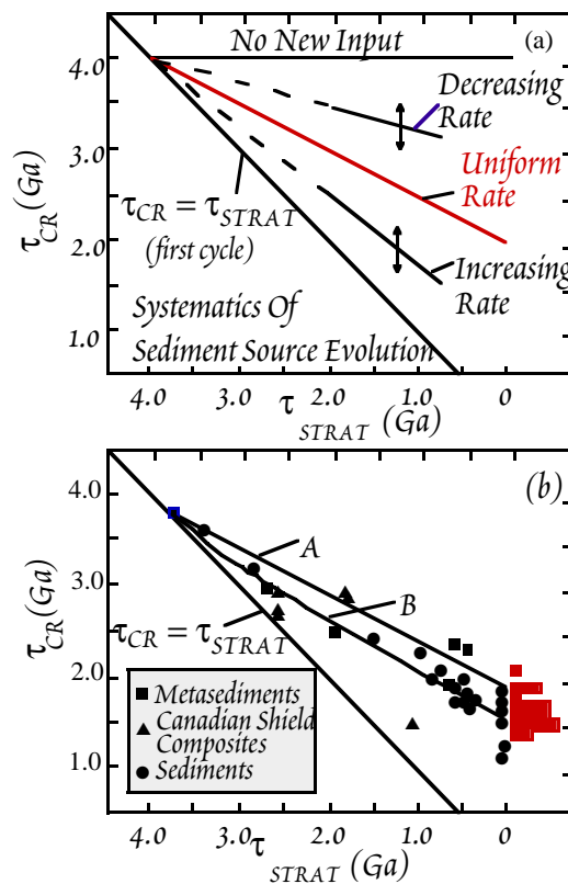
Figure 12.37. Relationship between stratigraphic age of sediments and the crustal residence age of material in sediments. From Goldstein et al., 1984).
