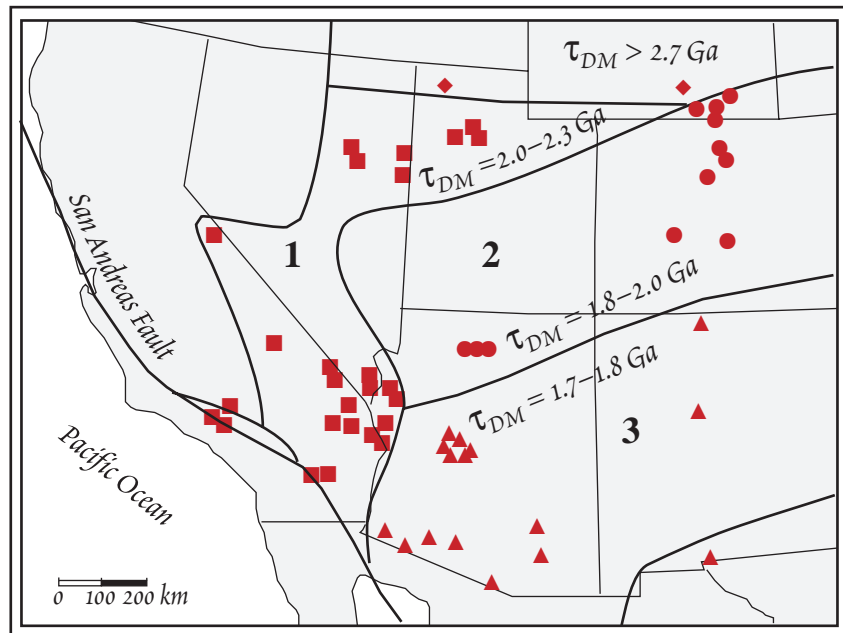
Figure 12.35. Isotopic provinces, based on crustal residence times ( \tau_{DM} ) of the Western U.S. From Bennett and DePaolo (1987).
