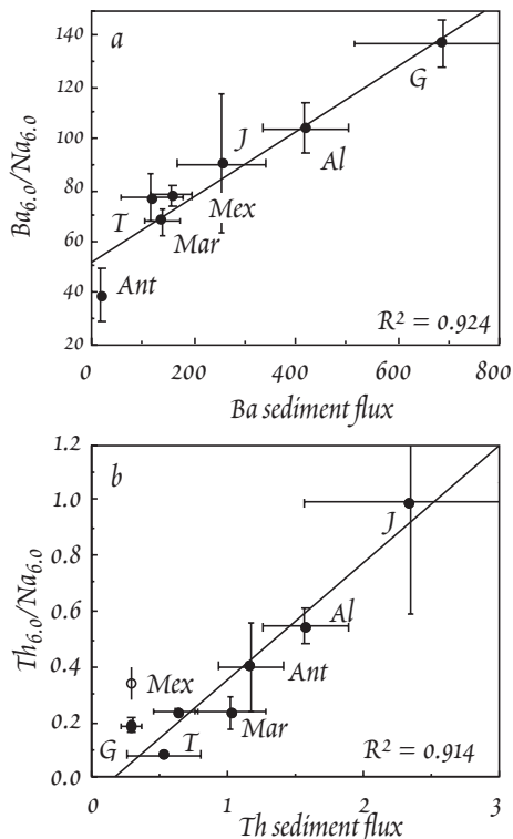
Figure 12.17. Relationship between Ba/Na_{6,0} and Th/Na_{6,0} in volcanics from 8 arcs and Ba and Th sediment flux beneath those arcs. Horizontal bars represent uncertainty in the amount of sediment subducted; vertical bars reflect the variance of the ratio in the arc volcanics. G is Guatemala, M: Mexico, J: Java, T: Tonga, Mar: Marianas, Al: Aleutians, Ant: Lesser Antilles. From Plank and Langmuir (1993).
