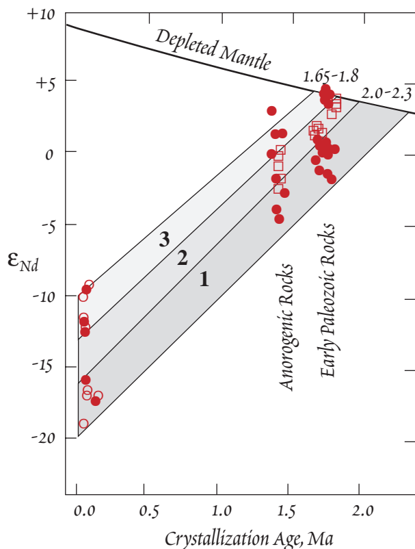
Figure 12.36. \epsilon_{Nd} (initial) as a function of crystallization age of Western U.S. Groupings 1, 2, and 3 refer to provinces shown in Figure 12.35. From Bennett and DePaolo (1987).
