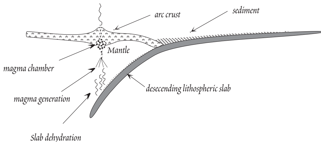
Figure 12.16. Cross-section of a subduction zone illustrating island arc magma genesis.
