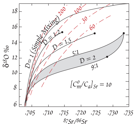
Figure 12.24. Variation of \delta^{18}\text{O} with ^{87}\text{Sr}/^{86}\text{Sr} during AFC for a magma with an initial \delta^{18}\text{O} = 5.7 and ^{87}\text{Sr}/^{86}\text{Sr} = 0.703 , and an assimilant with ^{87}\text{Sr}/^{86}\text{Sr} = 0.735 and \delta^{18}\text{O} = +19 . All curves are for R = 0.2 (5:1), except for one with D = 2 for which R = 0.11 (labeled 9:1). dashed lines are calculated Sr concentrations (ppm) assuming an initial concentration of Sr in the magma of 500 ppm. In the case where D = 1 , the problem simplifies to one of simple mixing. From Taylor (1980).
