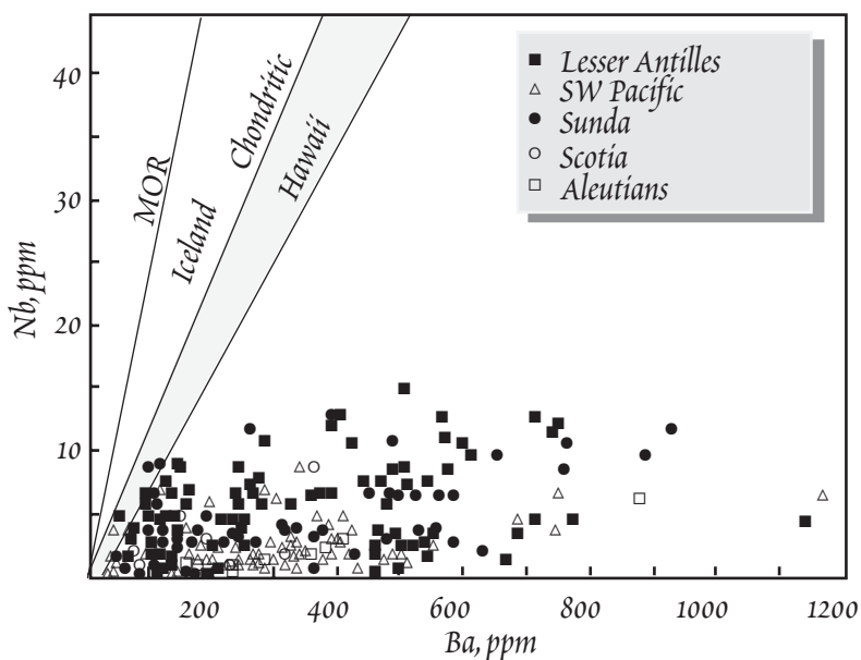
Figure 12.11. Low Nb concentrations of IAV compared to MORB and OIB illustrated by plotting Nb vs. Ba. From Perfit et al. (1980).
