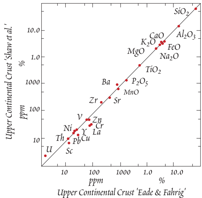
Figure 12.25. Comparison of estimates of the average composition of the upper crust by Eade and Fahrig (1971) and Shaw (1967). Both were based on studies of the Canadian shield, but different areas. From Taylor and McLennan (1985).
