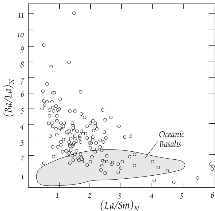
Figure 12.10. Relative alkali-alkaline earth enrichment of IAV illustrated by plotting the (Ba/La)_N ratio vs. the (La/Sm)_N ratio. The subscript N denotes normalization to chondritic values. From Perfit et al. (1980).
