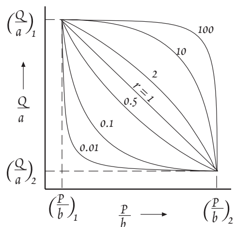
Figure 12.20. Plots of ratios of elements or isotopes, Q/a versus P/b for mixing of end members 1 and 2. The numbers along the curves are the values for r . From Langmuir et al. (1978).
