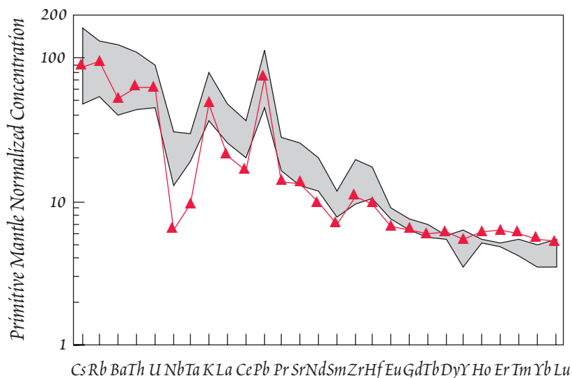
Figure 12.38. Comparison of incompatible element concentrations in a siliceous andesite from the Banda arc (red triangles) with the range of estimated concentrations in the continental crust (gray field). Both share a relative depletion in Nb and Ta and a relative enrichment in Pb.
