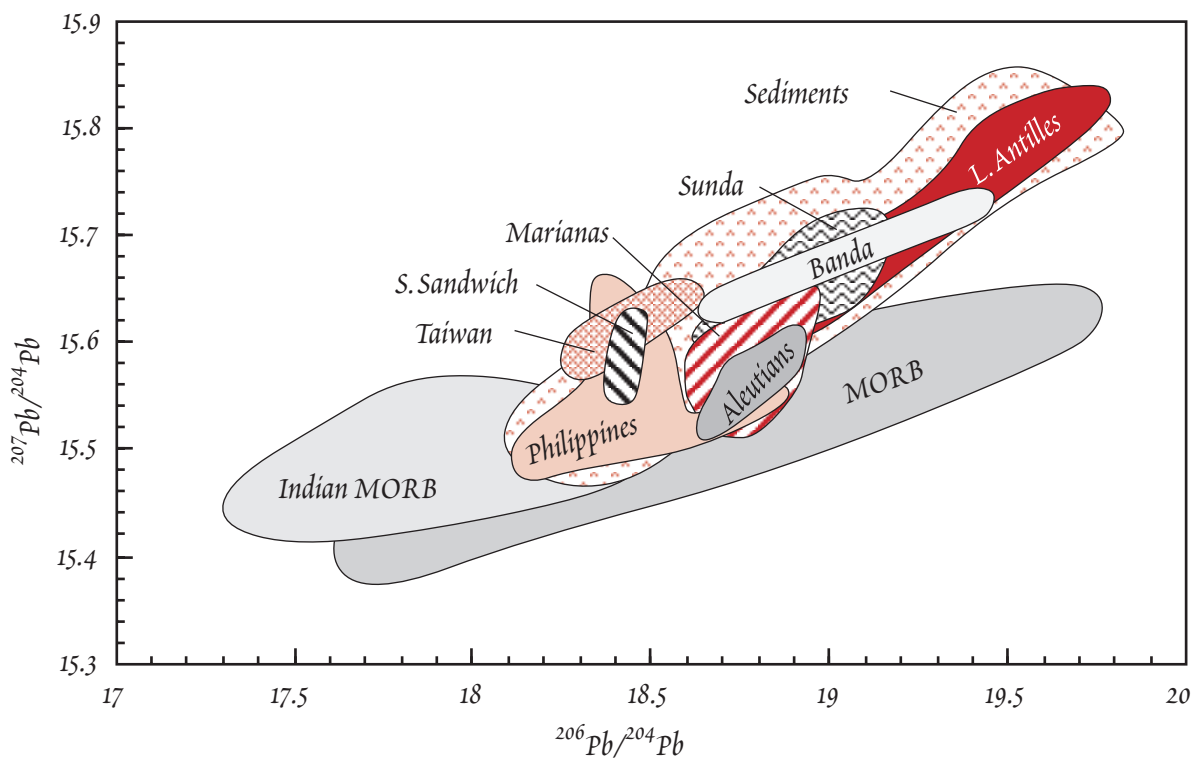
Figure 12.13. Pb isotope ratios in island arc volcanics. Fields for the South Sandwich, Lesser Antilles, Aleutians, Marianas, Philippines, Taiwan, Banda and Sunda arcs are shown and compared with fields for Atlantic and Pacific MORB (field labeled MORB) and Indian Ocean MORB (IMORB), and modern marine sediments.
