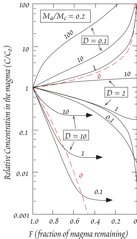
Figure 12.23. Variation of concentration during assimilation-fractional crystallization. Short dashed red lines are for simple fractional crystallization. Numbers on the curves refer to values of C_a/C_m^0 , the ratio of the concentration in the assimilant to the original concentration in the magma. After DePaolo (1981a).
