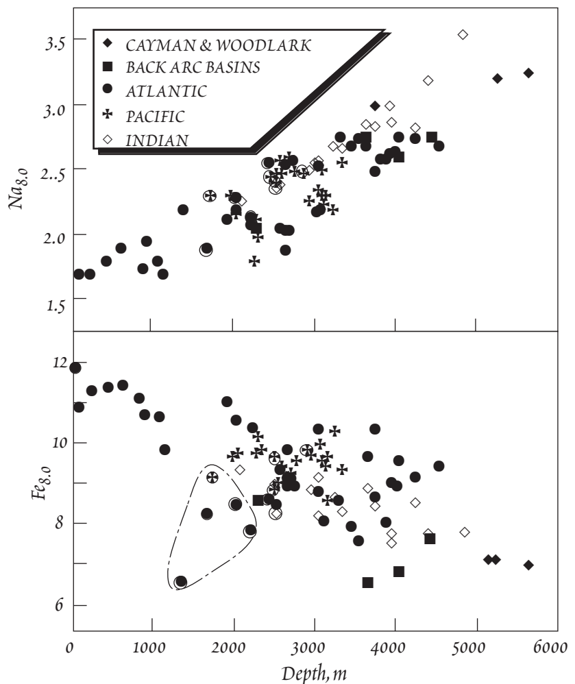
Figure 12.4. Relationship between Na_{8,0} and Fe_{8,0} in MORB and axial depth of mid-ocean ridges. Data from regions near hot spots are circled. Data from ridge segments near the Galápagos, Azores, and Jan Mayen hot spots, which are enclosed in the dashed field, appear to have anomalously low Fe. From Klein and Langmuir (1987).
