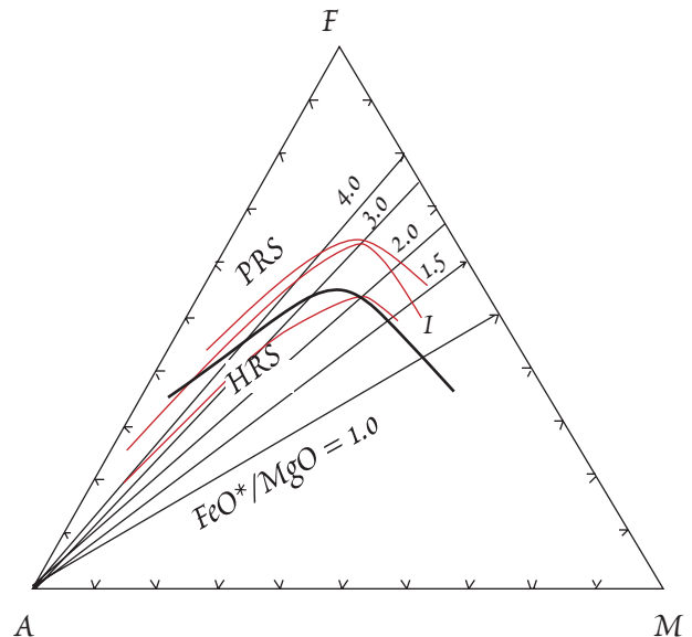
Figure 12.7 AFM (A=K 2 O+Na 2 O, F=FeO+MnO, M=MgO) diagram illustrating the difference between tholeiitic and calc-alkaline lava series of island arcs. Calc-alkaline rocks plot below the heavy line, tholeiites above. PRS is Kuno's pigeonite rock series; HRS is Kuno's hypersthene rock series. I is the Thingmuli series of Iceland. After Carmichael, et al. (1973).
