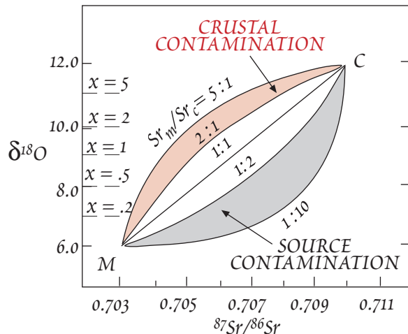
Figure 12.22. O—Sr isotope plot showing the difference is mixing curves produced by contaminating magma with crust (“crustal contamination”) as opposed to contaminating the magma source with subducted material (“source contamination”). x is the fraction of end member “C” (crust or subducted sediment) in the mixture. After James (1981).
