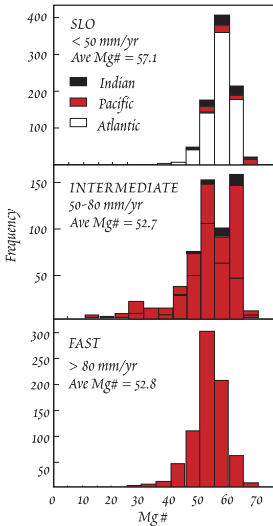
Figure 12.2. Mg# in basalts from mid-ocean ridges of differing spreading rates. The Mg# is used as an index of the extent of fractional crystallization. Because olivine is the primary crystallizing phase, and because the Mg# of olivine is much higher than that of the liquid, Mg# will decrease during fractional crystallization. The figure shows that basalts from slow spreading ridges experience somewhat less fractional crystallization on average than basalts from fast spreading ridges. The most fractionated basalts occur on intermediate spreading rate ridges where small discontinuous melt lens can occur. After Sinton and Detrick (1992).
