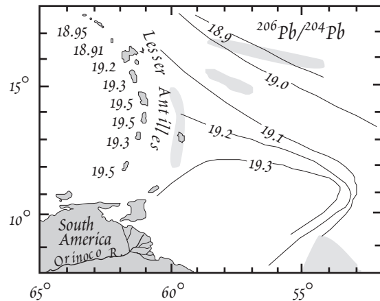
Figure 12.14. Pb isotope ratios in volcanics of the Lesser Antilles island arc and on the Atlantic Plate subducting beneath it. Contours show the ^{206}\text{Pb}/^{204}\text{Pb} ratios in the sediment, which increases from north to south due to the increasing contribution of Orinoco River sediment. The average ^{206}\text{Pb}/^{204}\text{Pb} for each island, which is shown beside the island, also increases from south to north. From White and Dupré (1986).
