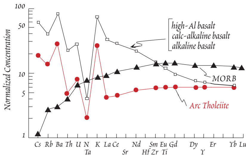
Figure 12.12. Spider diagram comparing typical incompatible element contents of island arc volcanics and MORB. Note the relative enrichment in alkalis and alkaline earths and the depletion in Ta in the island arc volcanics. After Sun (1980).
