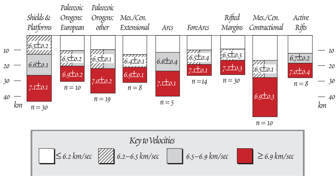
Figure 12.29. Seismic velocity structure of the continental crust, illustrating its 3-layered nature. Velocity structure falls into 9 types. The number of profiles used to construct each type is shown below each type. From Rudnick and Fountain (1995).
