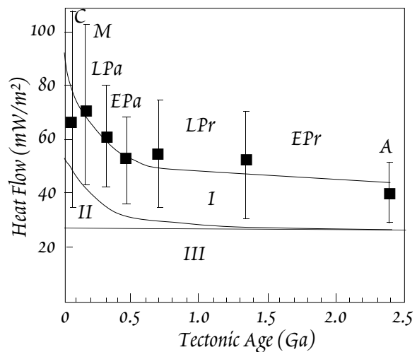
Figure 12.28. Heat flow as a function of tectonic age. Component I is radiogenic heat produced in the crust, II is heat from a transient thermal perturbation associated with tectonism, and III is background heat from deeper sources. A is Archean, EPr is Early Proterozoic, LPr is Late Proterozoic, EPa is early Paleozoic, LPa is late Paleozoic, M is Mesozoic, and C is Cenozoic. From Vitorello and Pollack (1980).
