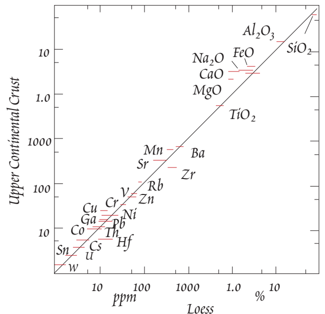
Figure 12.26. Comparison of elemental concentrations in loess with estimated upper crust. From Taylor and McLennan (1985).
