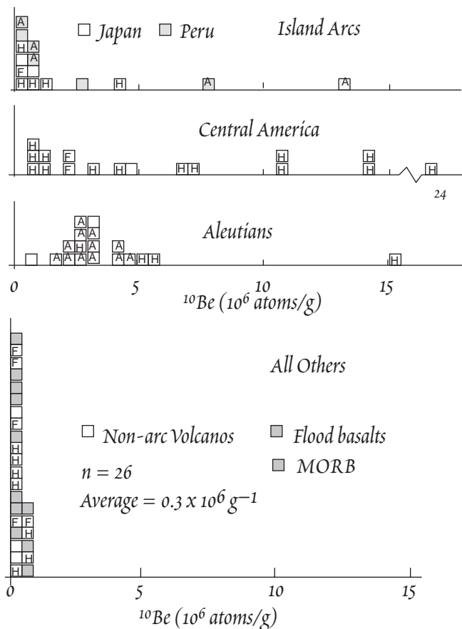
Figure 12.15. ^{10}\text{Be} in arc and non-arc lavas. "A" indicates sample from active volcano, "H" a historic eruption, and "F" (fresh) indicates collected during eruption. From Tera et al., 1986.
