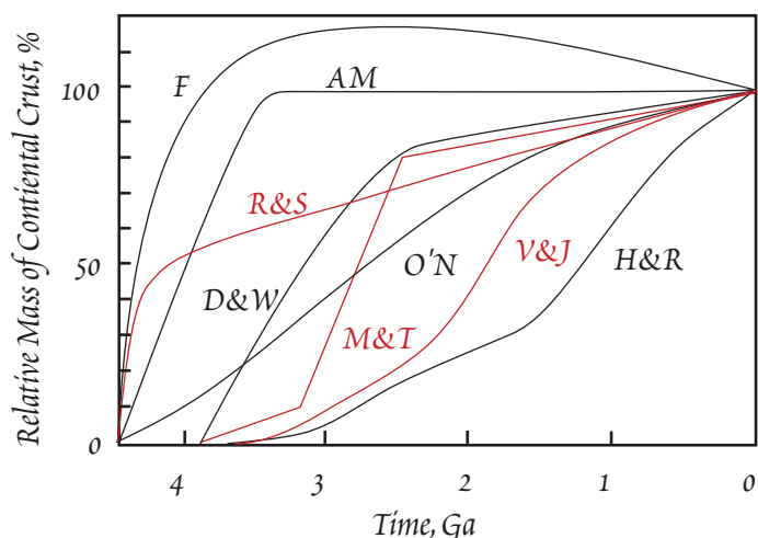
Figure 12.33. Models of the rates of crustal growth. AM: Armstrong (1981a), R&S: Rymer and Schubert (1984), F: Fyfe (1978), D & W: DePaolo and Wasserburg (1979), M & T: McLennan and Taylor (1982), O'N: O'Nions and Hamilton (1981), V & J: Veizer and Jansen (1979), H & R: Hurley and Rand (1969). Adapted from Taylor and McLennan (1985).
