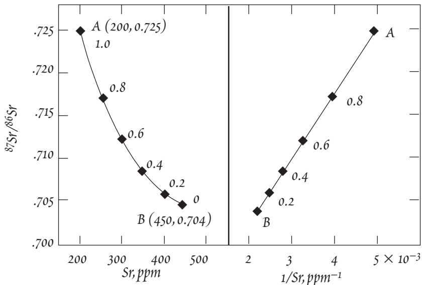
Figure 12.21. Mixing hyperbola formed by components A and B. After Faure (1986).
