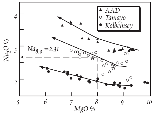
Figure 12.3. Na 2 O vs. MgO in MORB from three areas of the mid-ocean ridge system: the Australian-Antarctic Discordance, the Tamayo Fracture Zone area of the East Pacific Rise, and the Kolbeinsey Ridge, just north of Iceland. Thick arrows show calculated fractional crystallization paths ('liquid line of descent') for each data set. Na 8,0 values are the intersection of the fractional crystallization path with MgO concentration of 8%. This is illustrated for the Tamayo data (dashed lines), which has Na 8,0 of 2.31. After Klein and Langmuir (1987).
