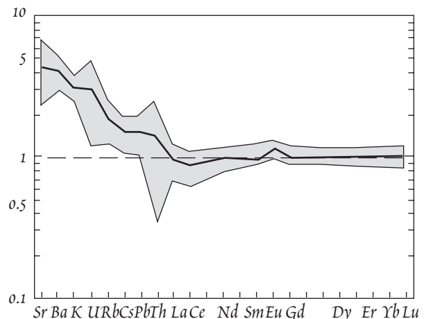
Figure 12.18. Ratio of observed enrichment of incompatible elements in Lesser Antilles low-K basalts compared to enrichment calculated from a sediment-depleted mantle mixing model based on Nd isotopic composition. Enrichment of the rare earths and Th can be accounted for by this model, but the enrichment of Pb, Cs, Rb, U, K, Ba, and Sr is greater than predicted, probably due to preferential transport of these elements in fluids. Gray area is 1 standard deviation of the basalts used in the average. From White and Dupré (1986).
