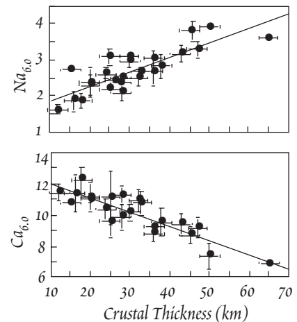
Figure 12.8 Correlation of Ca 6.0 and Na 6.0 with crustal thickness in island arc basalts. Ca 6.0 and Na 6.0 are the CaO and Na 2 O concentrations after correction for fractional crystallization to 6.0 MgO. From Plank and Langmuir (1988).
