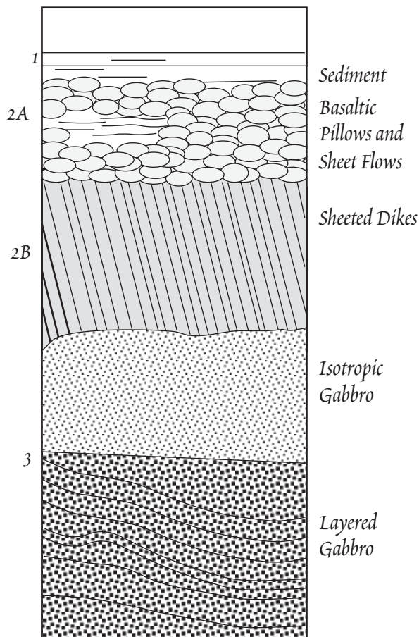
Figure 12.1. Schematic cross-section of the oceanic crust. Numbers on the left indicate the designation of seismically identifiable layers.
