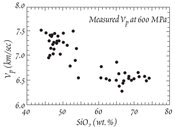
Figure 12.30. Correlation between measured seismic velocity ( v_p ) and \text{SiO}_2 concentration. From Rudnick and Fountain (1995).
