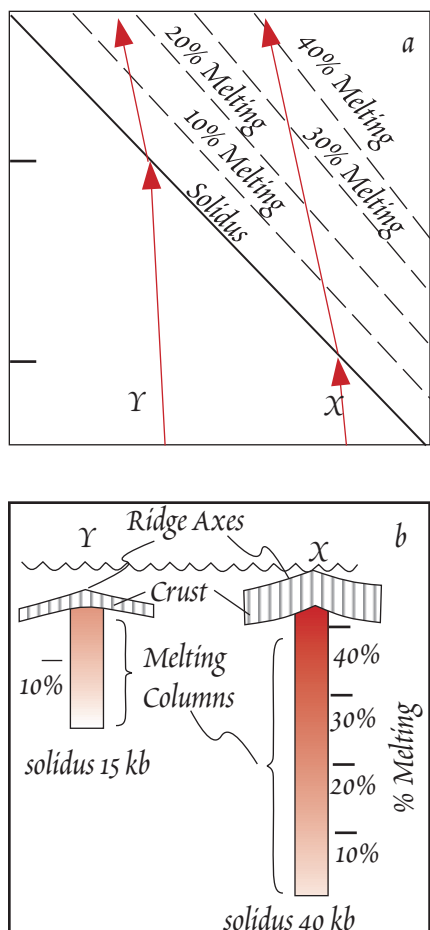
Figure 12.6. a.) Cartoon of the pressure-temperature relationship of adiabatically rising mantle undergoing melting. Hotter mantle (X) intersects the solidus at higher pressure and ultimately melts to a higher degree than cooler mantle (Y). The break in slope occurs because energy is consumed by melting (enthalpy of fusion). b.) Cartoon illustrating the relationship between axial depth, crustal thickness, melting, and mantle temperature. Hotter mantle (X) maintains the ridge at higher elevation because of its buoyancy. It also has a deeper melt column and melts to a greater degree, producing thicker crust than cooler mantle (Y). After Klein and Langmuir (1989).
