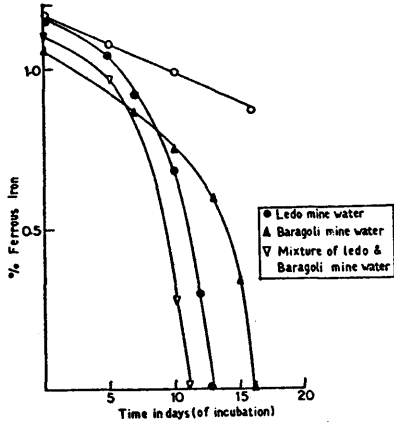
Fig.1 Decrease in Ferrous Iron conc. in media by growing culture of a) Iron & sulphur oxidising bacteria ▽ b) Iron oxidising bacteria ● ▲
