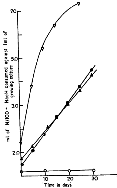
Fig. 3 Production of acid in media by a) iron & sulphur oxidising bacteria ∇ b) sulphur oxidising bacteria ● Δ
