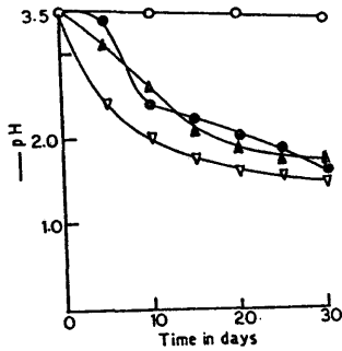
Fig. 2 Decrease in pH in media by a) iron & sulphur oxidising bacteria ∇ b) sulphur oxidising bacteria ● Δ
