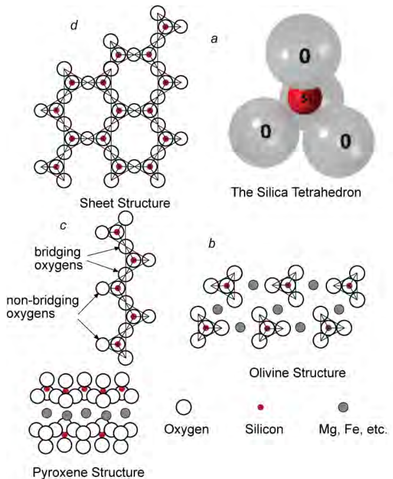
Figure 1.11. The silica tetrahedron and the structure of silicate minerals. a. The silica tetrahedron consists of a central silicon atom bound to 4 oxygens. b. In orthosilicates such as olivine, the tetrahedra are separate and each oxygen is also bound to other metal ions that occupy interstitial sites between the tetrahedra. c. In pyroxenes, the tetrahedra each share two oxygen and are bound together into chains. Metal ions are located between the chains. d. In sheet silicates, such as talc, mica, and clays, the tetrahedra each share 3 oxygens and are bound together into sheets.
