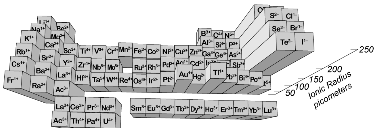
Figure 1.06. Ionic radii of the elements.
