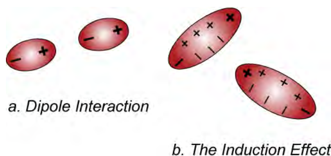
Figure 1.07. Van der Waals interactions arise because of the polar nature of some molecules. Illustrated here are (a) dipole-dipole interactions, which occur when two dipolar molecules orient themselves so oppositely charged sides are closest, and (b) the induction effect, which arise when the electron orbits of one molecule are perturbed by the electromagnetic field of another molecule.
