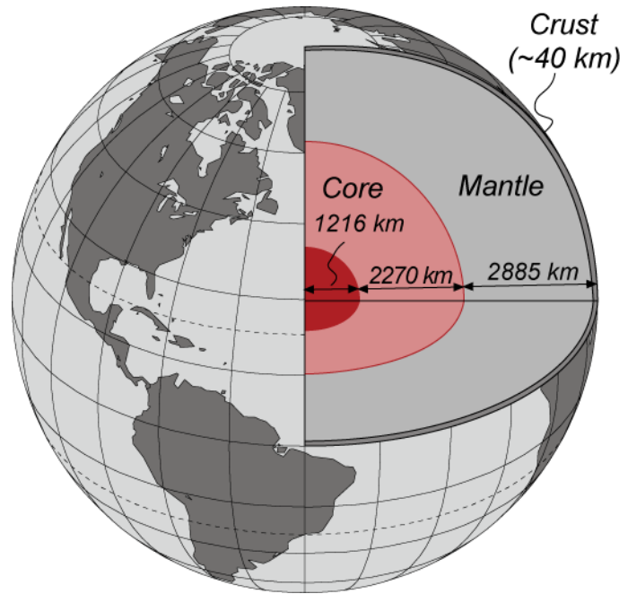
Figure 1.09. The Earth in cross-section. The outer rocky part of the planet, the mantle and crust, consists principally of silicates and is 2885 km thick. The core, divided into a liquid outer core and a solid inner core, consists of iron-nickel alloy and is 3486 km thick.
