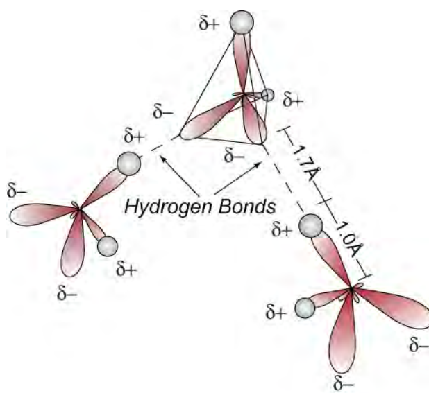
Figure 1.08. Hydrogen bonding between water molecules. Hydrogen positions shown as red; sp^3 hybrid orbitals in oxygen shown as dark gray. The \delta+ and \delta- indicate partial positive and negative charges respectively.
