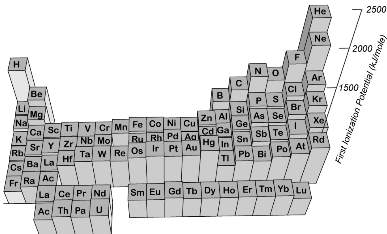
Figure 1.04. First ionization potential of the elements.
